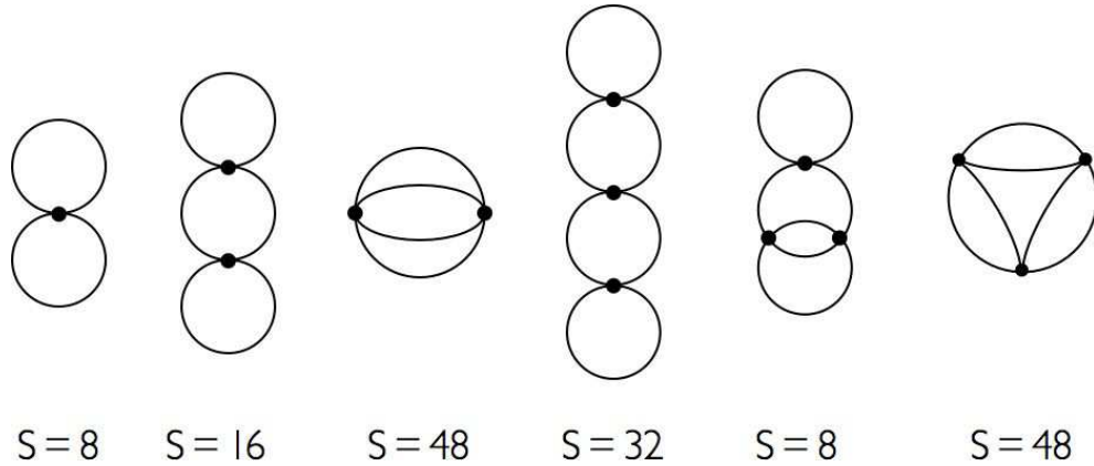
Figure 1.17: Cluster symmetry factors for the quartic theory. A vertex is represented as a black dot ( \bullet ) with four 'legs'.
