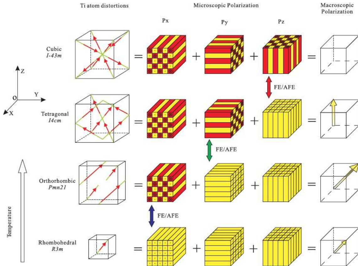
Figure 6.10: Fig. 1 from Zhang, Cagin, and Goddard (2006) showing \text{Ti}^{4+} ion distortions and polarizations in \text{BaTiO}_3 , as determined from density functional calculations.
