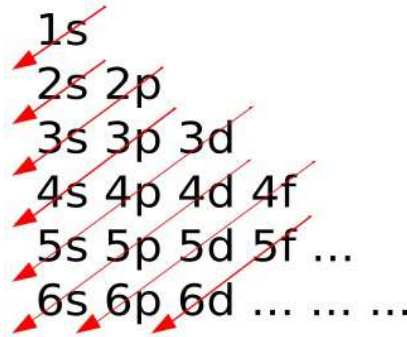
Figure 6.1: The Aufbau principle and the diagonal rule. Image credit: Wikipedia.
