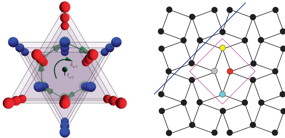
Figure 5.11: Two nonsymmorphic crystal lattices. Left: The hexagonal close packed lattice (space group P6_3/mmc ) has a two site unit cell (red and blue) and a screw axis symmetry, given by a rotation by 60^\circ followed by a translation of \frac{1}{2}\mathbf{a}_3 along the c -axis. The underlying Bravais lattice is simple hexagonal. Right: The Shastry-Sutherland lattice (space group p4g ) has a four site unit cell (shown in center) and a glide mirror (blue line). Translation by half a unit cell along the mirror line followed by a mirror reflection is a lattice symmetry. The underlying Bravais lattice is square.
