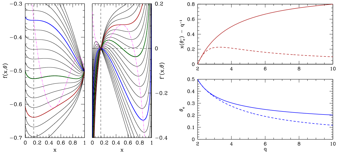
Figure 7.20: The left panels show the variational free energy f(x, \theta) of the q = 7 state Potts model and its x -derivative f'(x, \theta) versus the variational parameter x , for a set of equally spaced temperatures. The vertical dashed black line is at x = q^{-1} = \frac{1}{7} . The dot-dash magenta curve in both cases is the locus of points for which the second derivative f''(x, \theta) with respect to x vanishes. Three characteristic temperatures are marked: (i) \theta = q^{-1} (blue), where the coefficient of the quadratic term in the Landau expansion changes sign, (ii) \theta = \theta_0 (red), where there is a saddle-node bifurcation and above which the free energy has only one minimum at x = q^{-1} (symmetric phase), and (iii) \theta = \theta_c (green), where the first order transition occurs. The right panels show comparisons of the order parameter jump at \theta_c (top) and critical temperature \theta_c (bottom) versus q for untruncated (solid lines) and truncated (dashed lines) expansions of the mean field free energy. Note the agreement as q \rightarrow 2 , where the jump is small and a truncated expansion is then valid.
