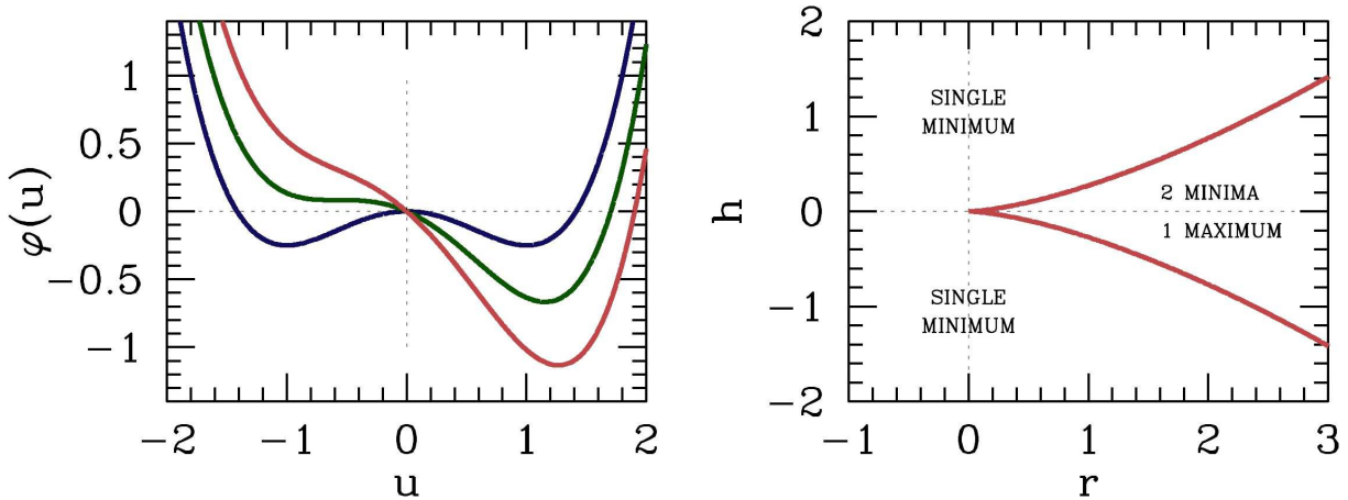
Figure 7.29: Left: scaled free energy \varphi(u) = -\frac{1}{2}ru^2 + \frac{1}{4}u^4 - hu , with h = 0 (blue), h = h_c (green), and h = 2h_c (red), where h_c = \frac{2}{3\sqrt{3}}r^{3/2} . Right: phase diagram for the imperfect bifurcation \dot{u} = -\varphi'(u) = h + ru - u^3 in the (r, h) plane.
